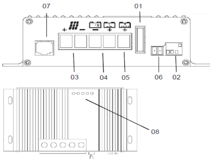
Fig 1: Device elements
